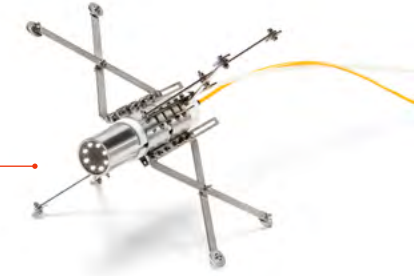
Horizontal centering device for horizontal use - with regulation Ø105-332mm Protects the camera head from accidental shocks and keeps it centered in the hole
