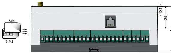
Drawings and dimensions (all dimensions in millimeters)
